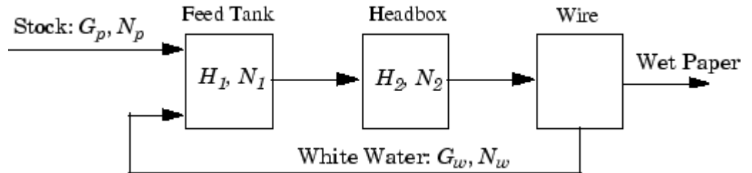
Schematic of Paper Machine Headbox Elements
